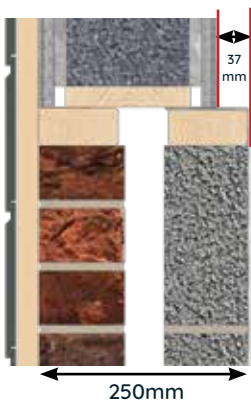
hup! on 250mm existing wall - full clad
