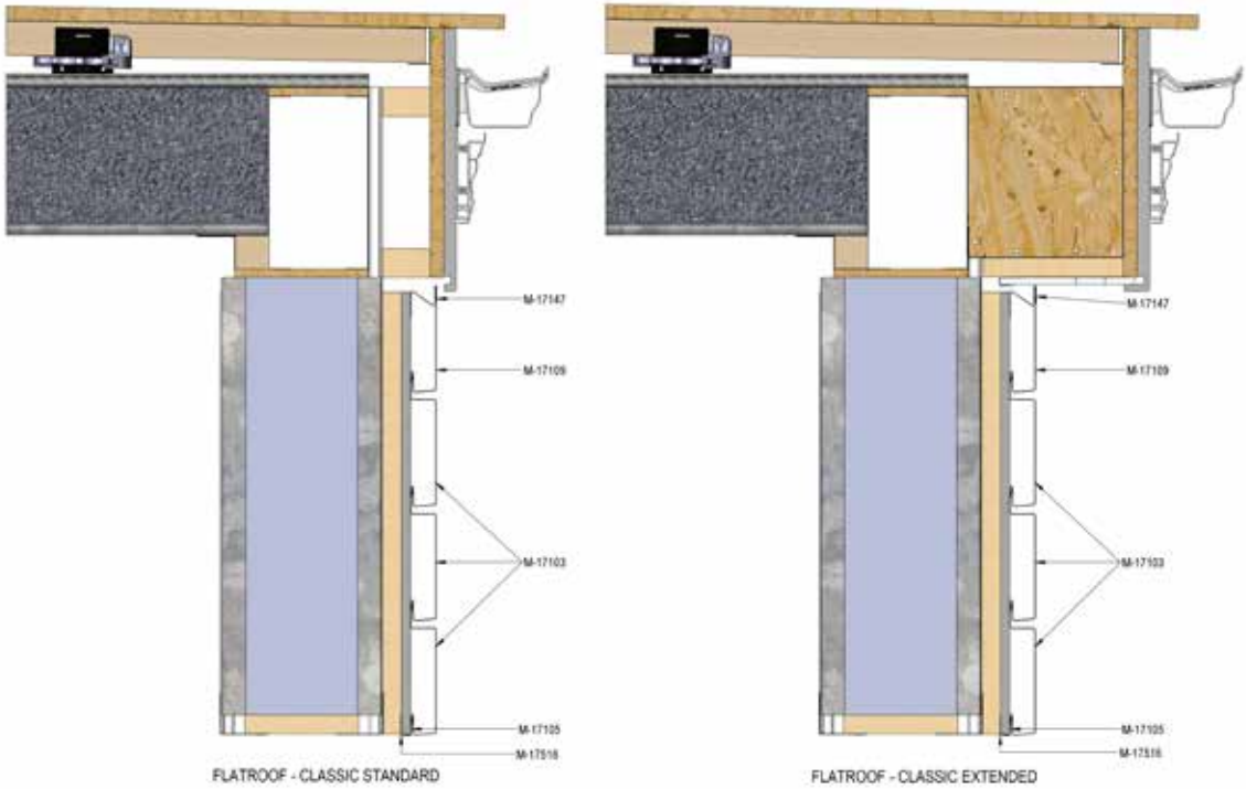
Flat Roof classic with steel facade
