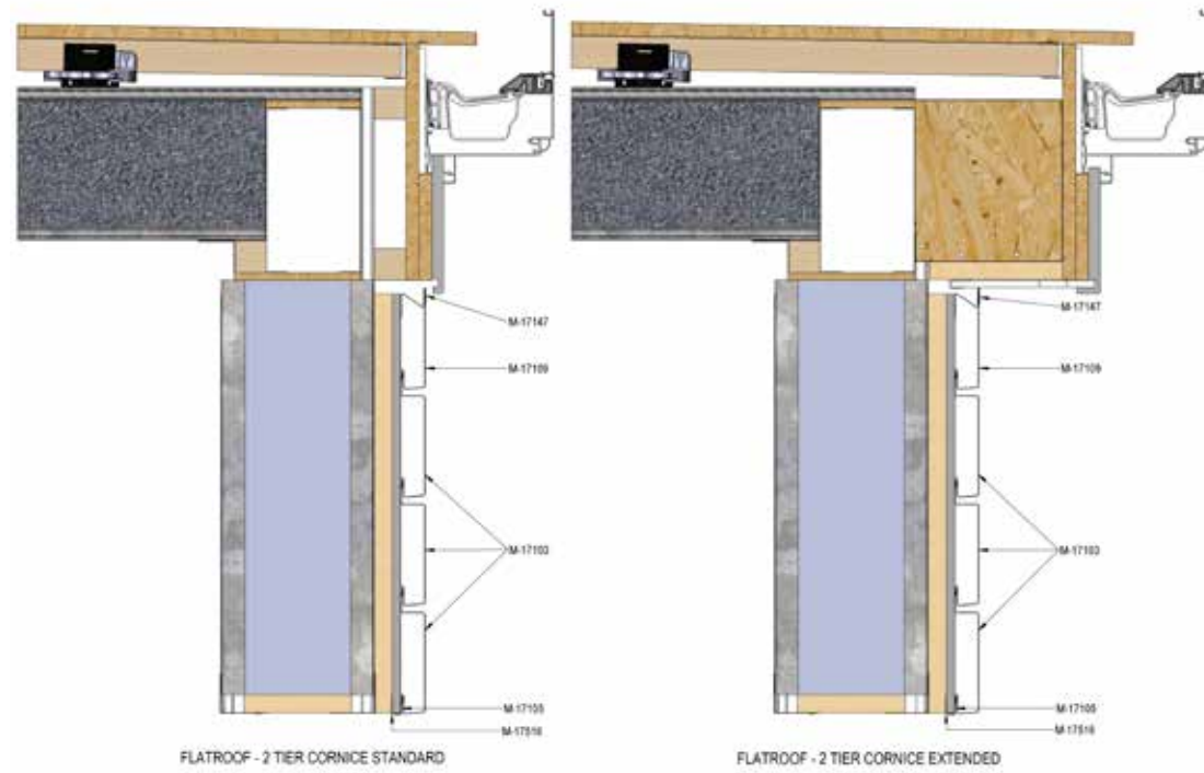
Flat Roof 2 tier with steel facade
