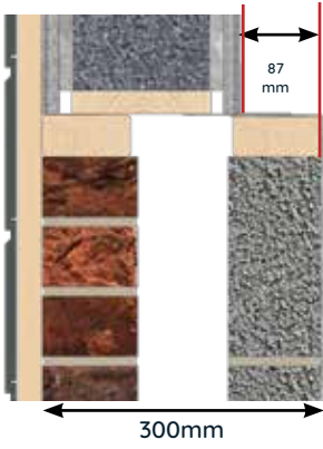
hup! on 300mm existing wall - full clad
