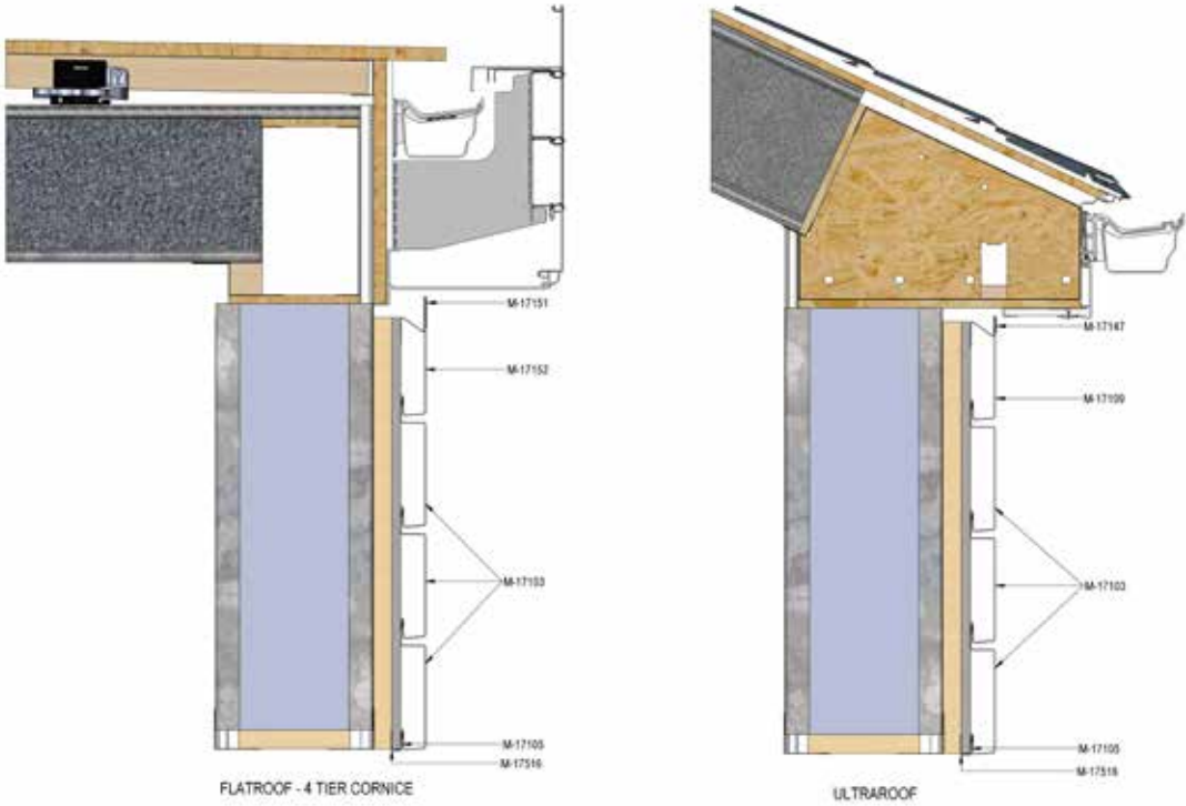
4 tier and Ultrarroof with steel facade
